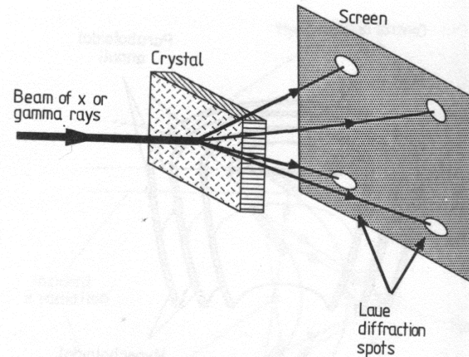
Figure 1.3.12. Laue diffraction of x- and gamma rays.
