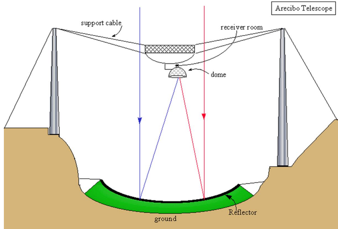
A 305 m spherical reflector
